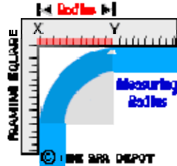
Figure 1a. Measuring the radius of a curve.
